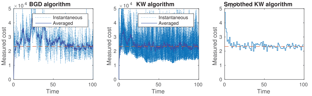
Fig. 11. Cost evolution vs. time for the online optimization algorithms analyzed.
